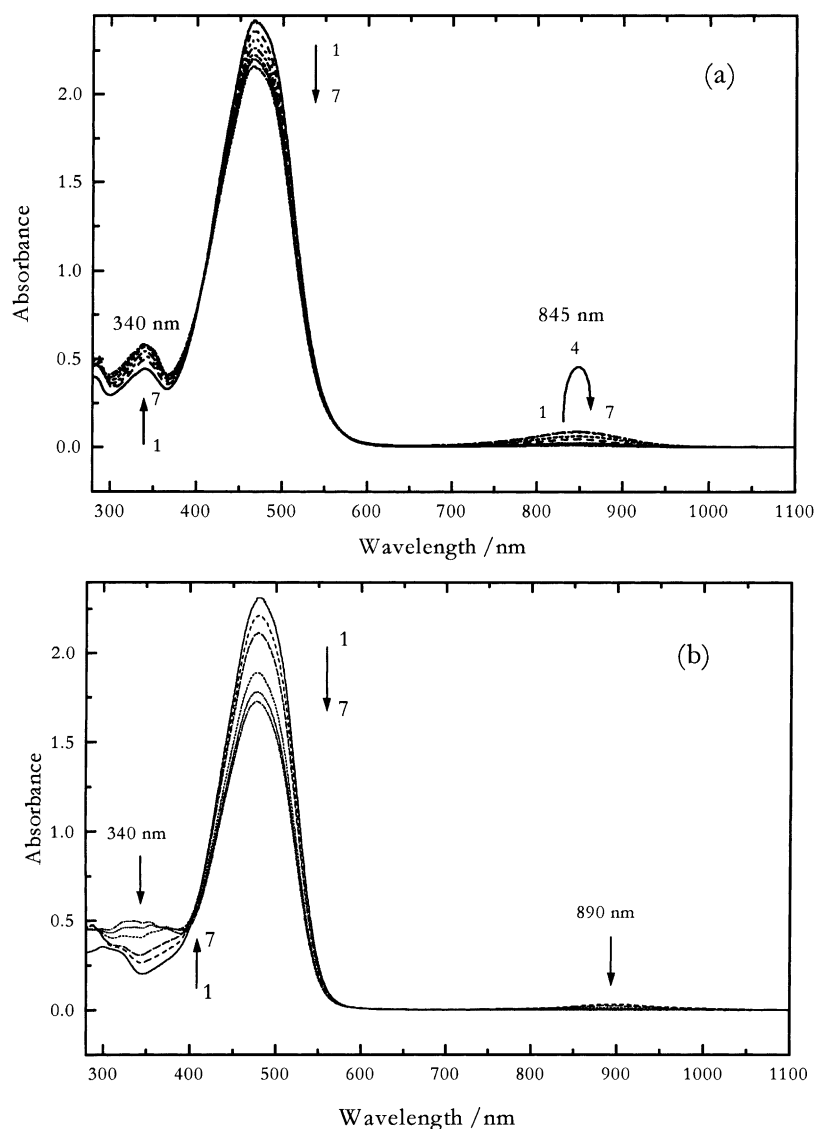
Fig. 3. UV-VIS spectra of the mixture of (a) 0.02 mM 8'-apo-β-caroten-8'-al and 0.02 mM DDQ solutions in CH 2 Cl 2 : (1) carotenoid only; (2) +DDQ; (3) after 2 min; (4) after 5 min; (5) after 10 min; (6) after 20 min; (7) after 60 min and (b) 0.02 mM canthaxanthin and 0.02 mM DDQ solutions in CH 2 Cl 2 : (1) carotenoid only; (2) +DDQ; (3) after 2 min; (4) after 5 min; (5) after 10 min; (6) after 20 min; (7) after 50 min.
