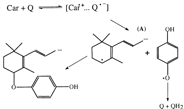
Scheme 3. Diamagnetic product formation.
